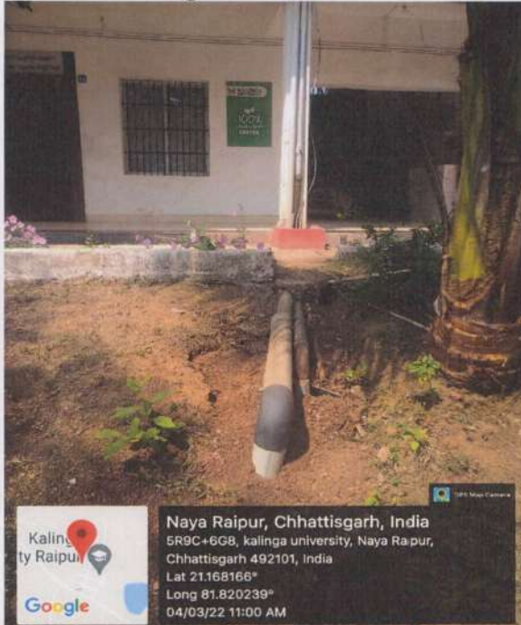
Soak Pit to harvesting Rain Water No-02
